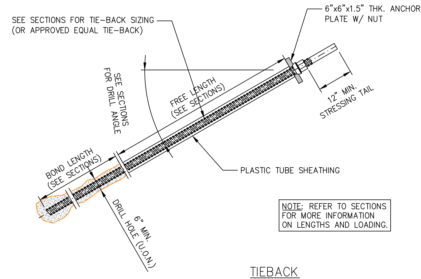
TIEBACK
